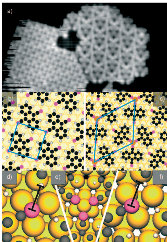
Figure 2. a) STM image of DCA on Cu(111) obtained at 180 K ( 175 \times 95 Å, -2.6 V, 0.22 nA), depicting separate regions of the \alpha phase (left) and \beta phase (right). b), c) DFT minimization of the adsorbate patterns ( \alpha and \beta phase) with the unit cell indicated. Because the unit cell in (c) is more than three times larger, only two substrate layers were included. d) Hydrogen bonding in the \alpha phase. e) Coordination of a Cu adatom in the \beta phase. f) Increased N...H-C length in the \beta phase indicating the absence of hydrogen bonding. The calculations for the \alpha and \beta phases used two and three substrate layers, respectively, leading to the difference in apparent background of panels (d), (e), and (f). Key as for Figure 1.
