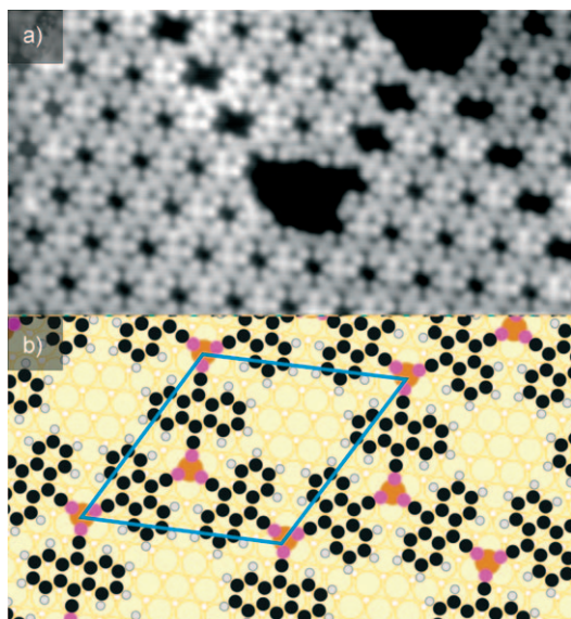
Figure 3. a) STM image ( 180 \times 100 \text{ Å} , -3.8 \text{ V} , 57 \text{ pA} , 30 \text{ K} ) of the \gamma phase of DCA on Cu(111). b) Corresponding model. Key as for Figure 1.
